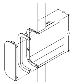
Passante fianco terminale cestoni base / Double horizontal groove at end of side panel / Traversant grands bacs de base.
